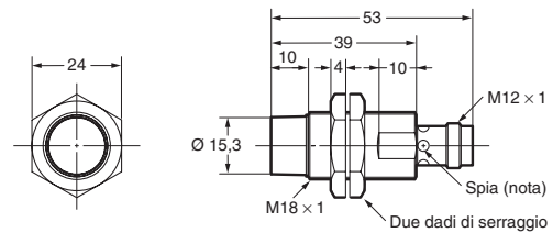
E2A-M18KN16-M1-□□/E2A-S18KN16-M1-□
