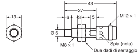
E2A-S08KN04-M1-□□
