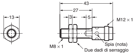
E2A-S08KS02-M1-□□
