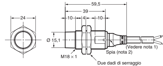
E2A-M18KN16-WP-□□/E2A-S18KN16-WP-□
